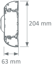
Medical gas casing with fitting up and down
