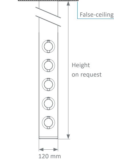
Medical gas casing without fitting
