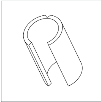
Adapter Ø30 for tube Ø38 Ref : 510088
