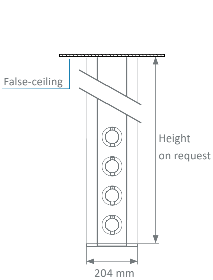
Medical gas casing with fitting
