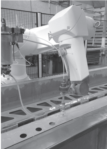
Aluminum machining Water jet machine - RX160
