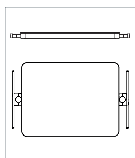
Tray 605x455 mm with lateral rails (50 kg max)
