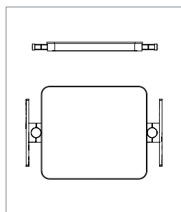
Tray 405x355 mm with lateral rails (40 kg max)
