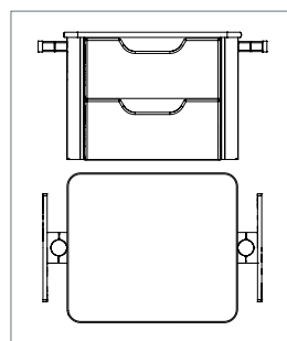
Tray unit 405x355 mm with double drawer and with lateral rails (40 kg max)
